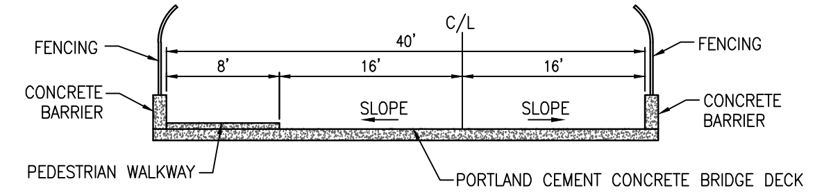
CROSS SECTION 'X'
