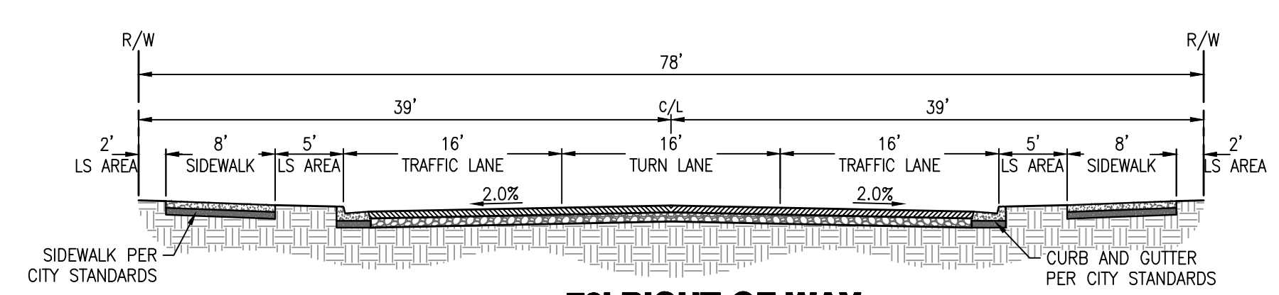
A 78' RIGHT-OF-WAY PORTION OF STREET "A" NOT TO SCALE
