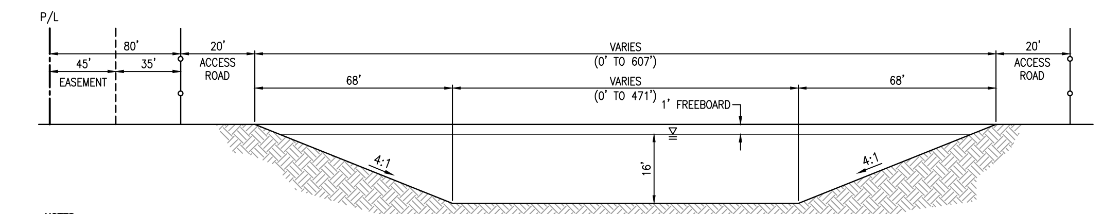
E BASIN CROSS SECTION E NOT TO SCALE
