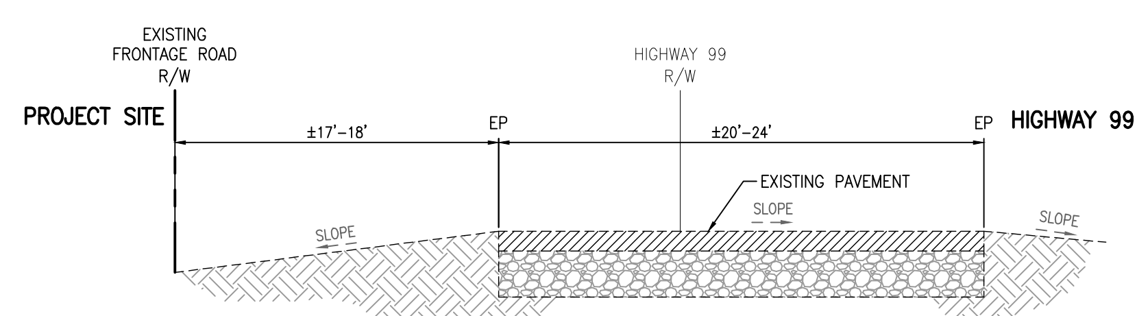
G EXISTING SOUTH STATE ROUTE 99 FRONTAGE ROAD NOT TO SCALE
