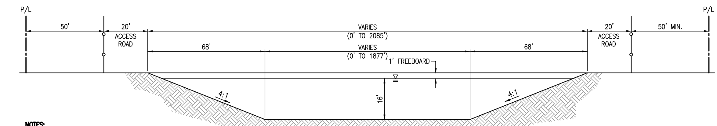
D BASIN CROSS SECTION D NOT TO SCALE
