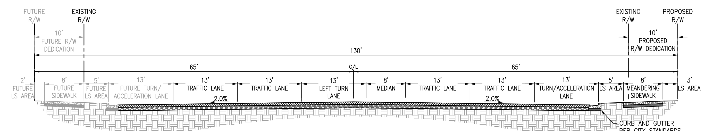
C 130' RIGHT-OF-WAY AIRPORT WAY NOT TO SCALE
