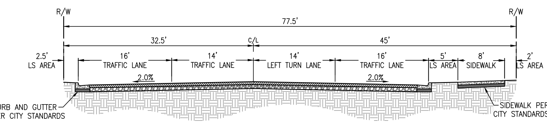
B 77.5' RIGHT-OF-WAY PORTION OF STREET "A" NOT TO SCALE
