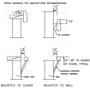
FIGURE 32A HANDRAIL MOUNTING EXAMPLES
