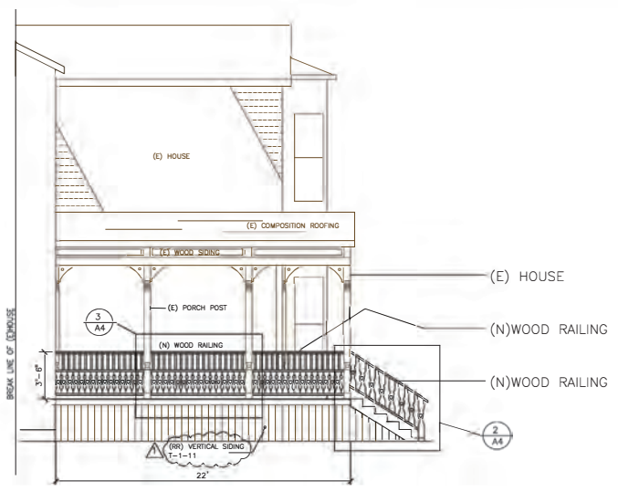
SIDE ELEVATION (EAST) 1/4" = 1'-0"
