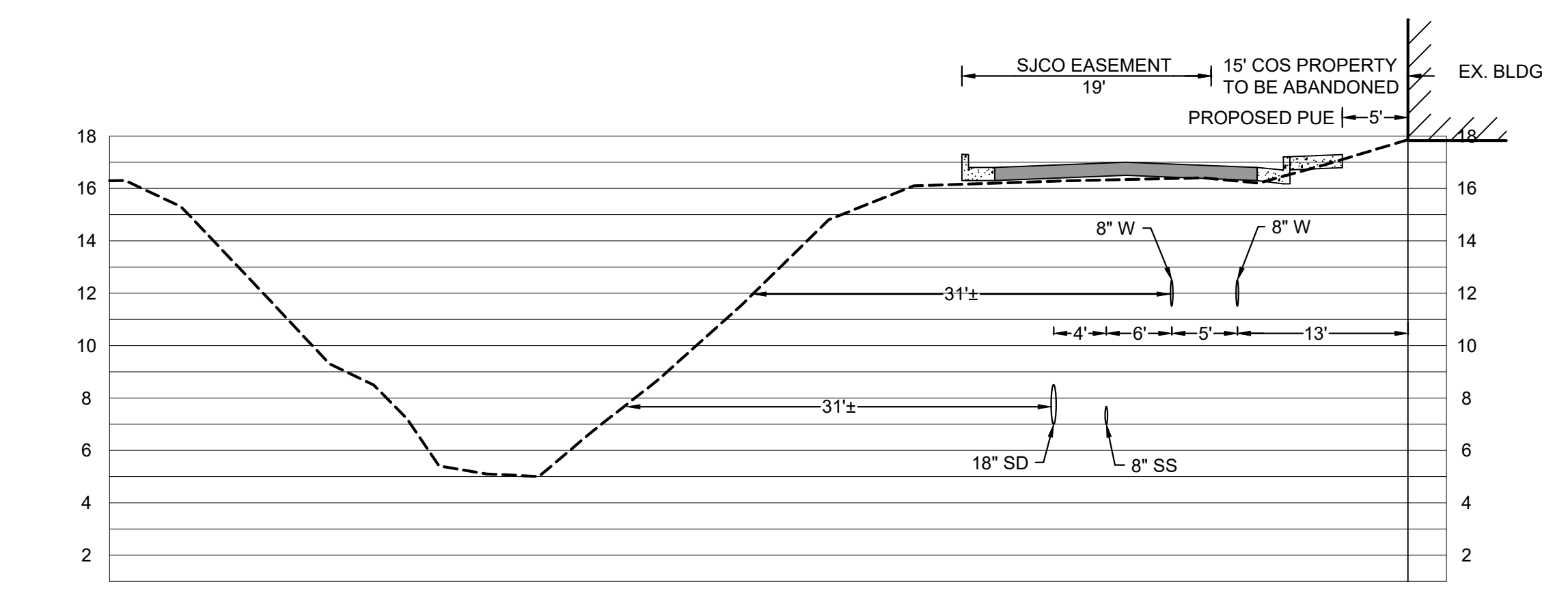
SECTION B - B SCALE: HORIZONTAL: 1" = 10' VERTICAL: 1" = 5'
