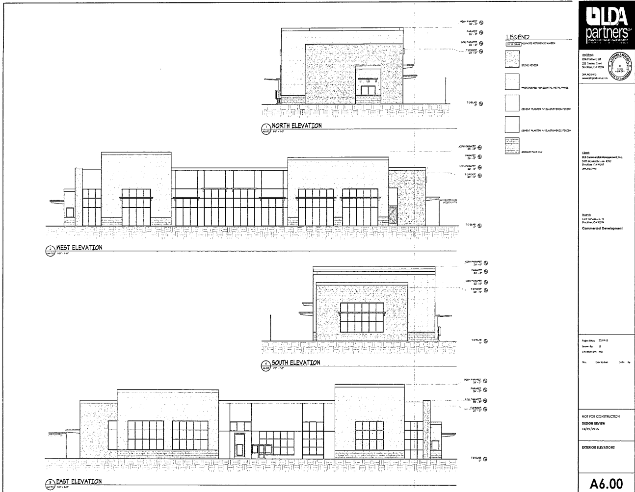
Elevations
