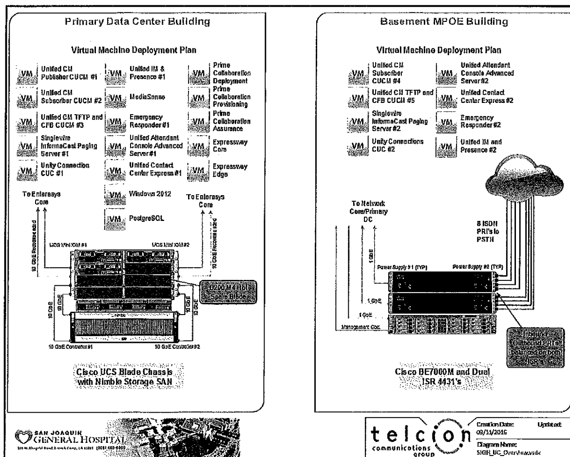
Figure 0.2 - SJGH UC Design Overview
