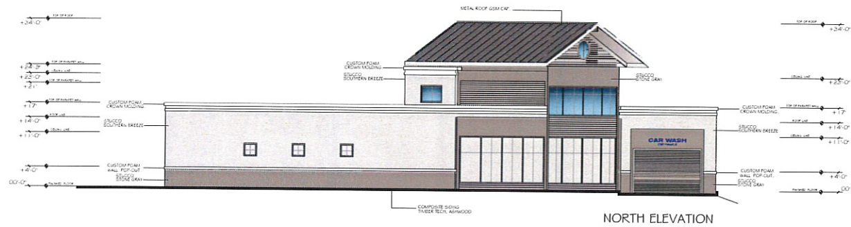
NORTH ELEVATION
