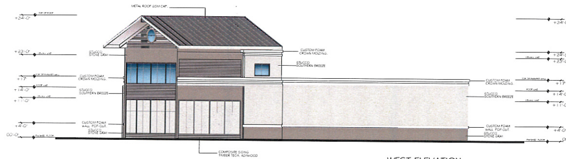
WEST ELEVATION
