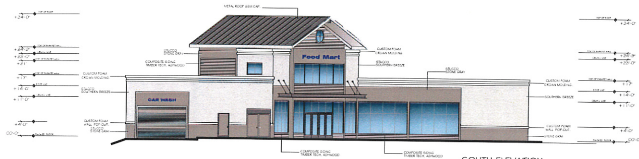
SOUTH ELEVATION
