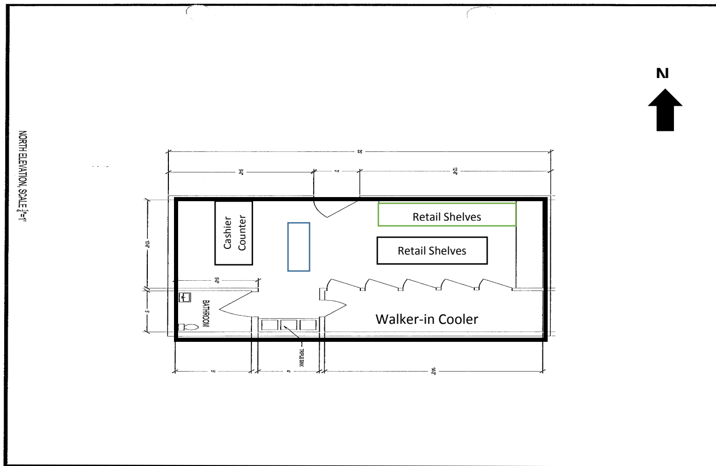
Floor Plan
