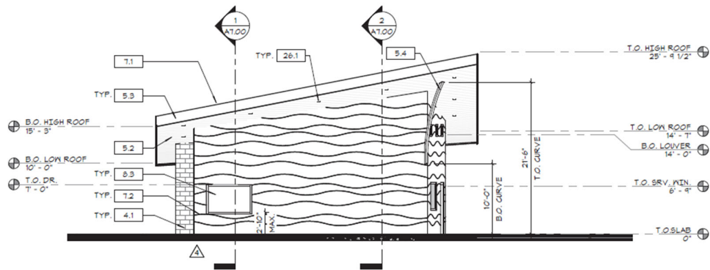
2 EXTERIOR ELEVATION - WEST A6.00 1/8" = 1'-0"
