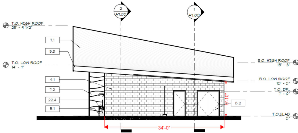
1 EXTERIOR ELEVATION - EAST A6.00 1/8" = 1'-0"
